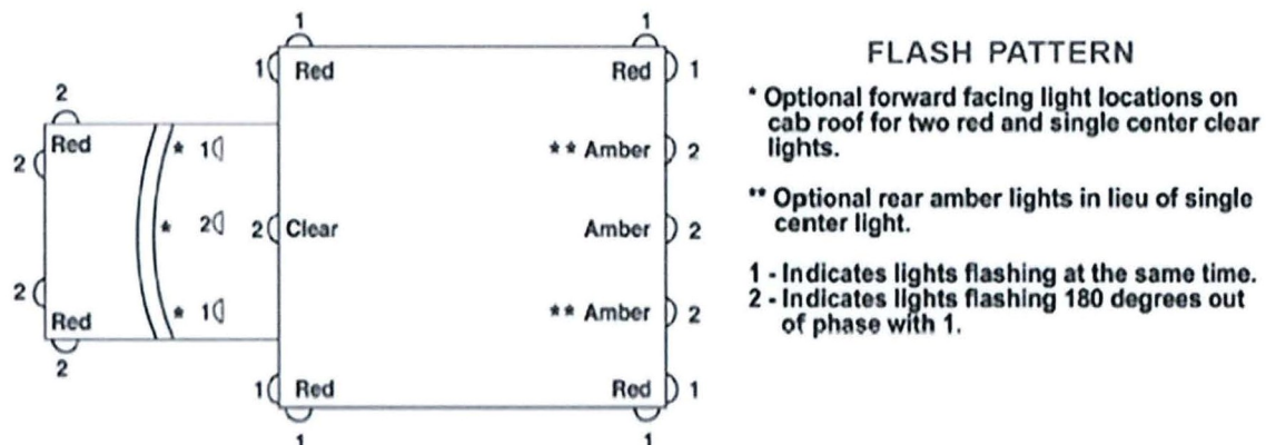
Figure 1 – Emergency Lighting
