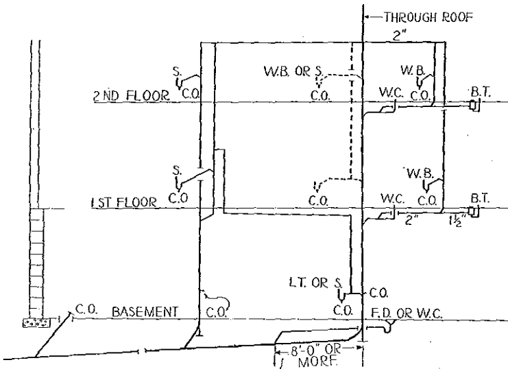
(7) Illustrating minimum requirements for a two-story residence or similar installation. H 62.06 (1), H 62.07 (6), (7) (b).
