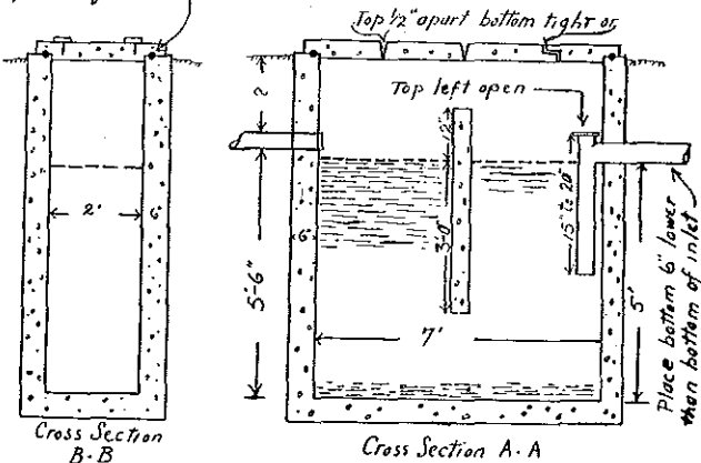
(28) Showing the design of a large grease basin in connection with hotels, restaurants or institution kitchens. H 62.11 (2) (b).
