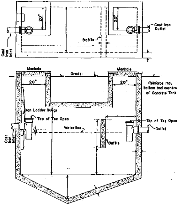
CROSS SECTION OF SEPTIC TANK
