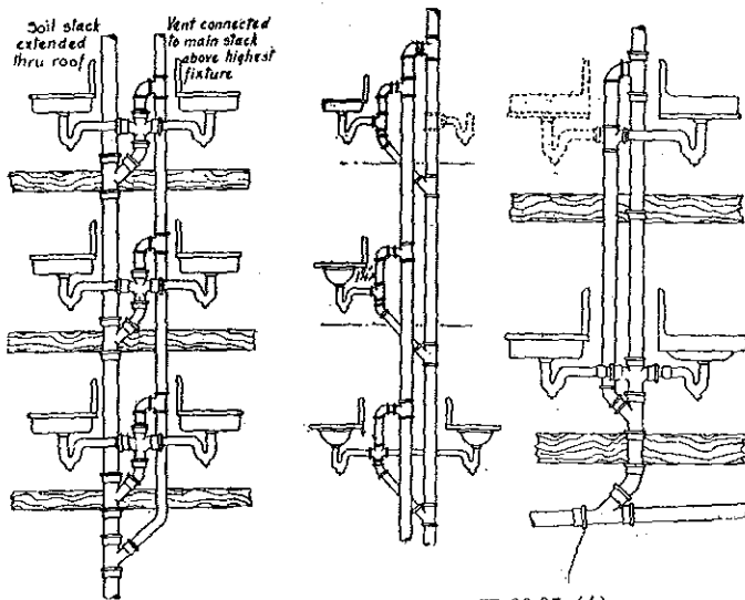
(14) Illustrating provisions of H 62.07 (4).
