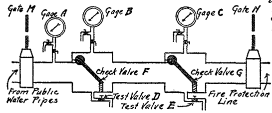
Fig. 3 Arrangement Diagram of Valves
