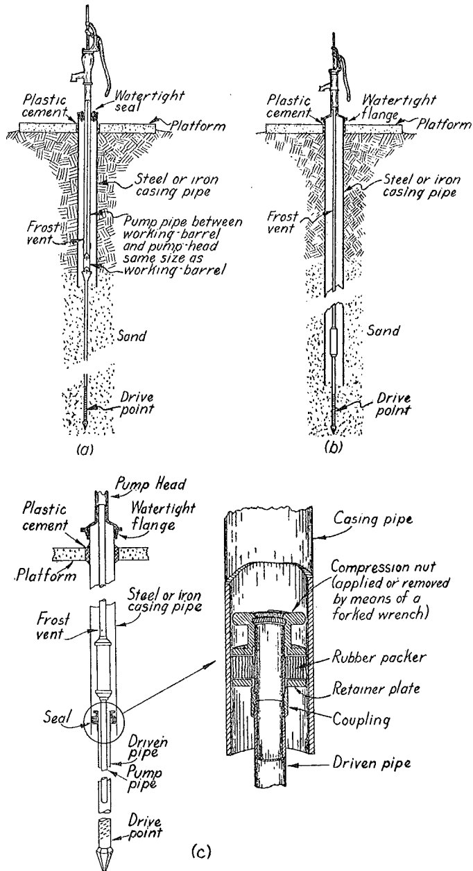
Figure 7. Driven Point Well Construction. Illustration (c) shows suitable method of returning frost drain water to well when impervious soil is present. See Wis. Adm. Code section NR 112.05 (5).
