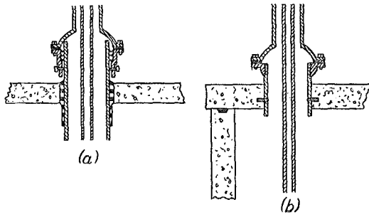
Figure 10. Hand Pump Mountings. (a) On well casing pipe through a water-tight pump flange. (b) On a section of pipe set in concrete well top and fitted with a pipe flange. See NR 112.09 (1) and (2) (a).
