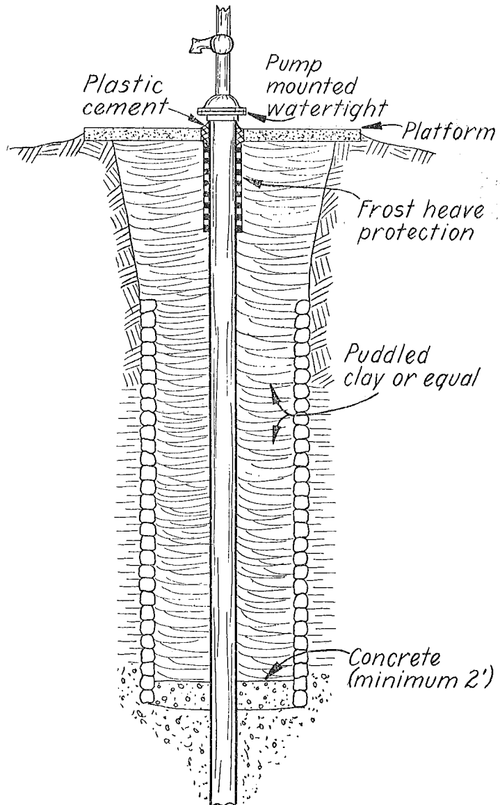
Figure 9. Drilled Well Constructed in Existing Dug Well. See Wis. Adm. Code section NR 112.05 (7).
