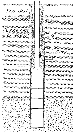
Figure 6. Bored Type Well Construction. See Wis. Adm. Code section NR 112.05 (4).
