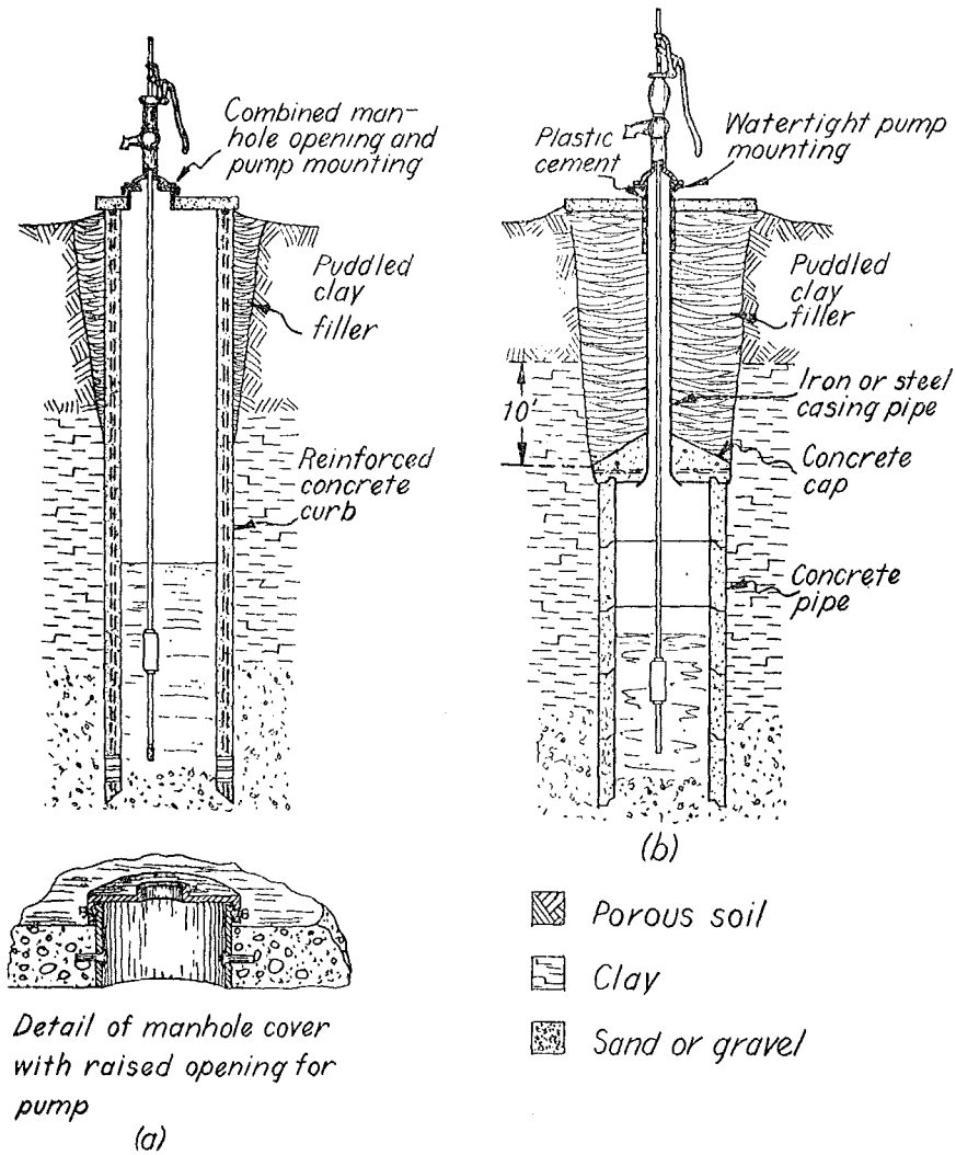
Figure 8. Sanitary Construction of Dug Wells. See Wis. Adm. Code Section NR 112.05 (6).
