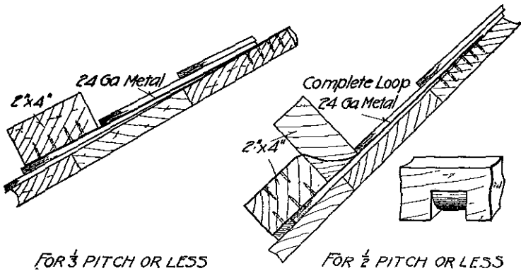
Fig. 11.—Roofing Scaffolds
