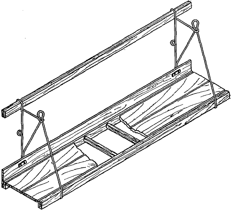
Fig. 9.—Swinging Scaffold
