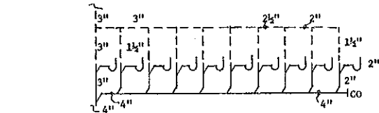
2" TRAP SERVING 2 WASHERS—20 TOTAL—2 EACH TRAP
