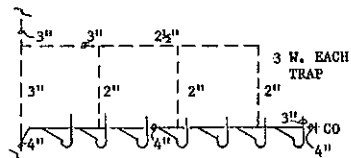
3" TRAP SERVING 3 WASHERS
