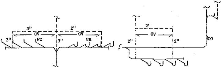
CV = CIRCUIT VENT
