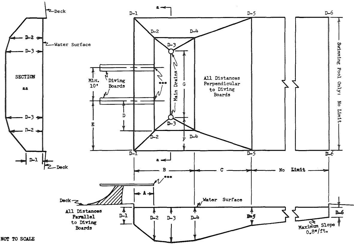
FIGURE I PLAN and PROFILE SWIMMING POOL and DIVING BOARD INSTALLATION
