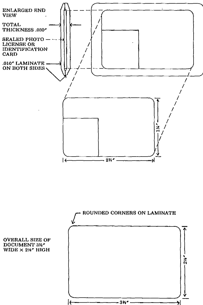
FIGURE 3 Laminate Specifications
