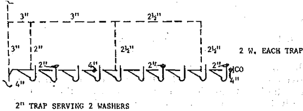
2" TRAP SERVING 2 WASHERS
