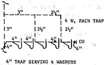
4" TRAP SERVING 4 WASHERS
