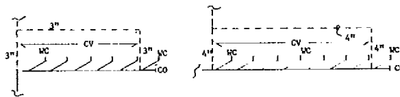
CV = CIRCUIT VENT
