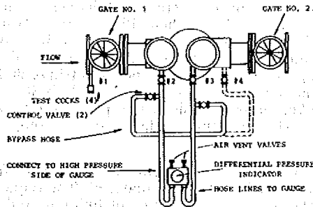
DIFFERENTIAL PRESSURE INDICATOR METHOD FOR REDUCED PRESSURE BACKFLOW PREVENTERS
