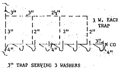
3" TRAP SERVING 3 WASHERS
