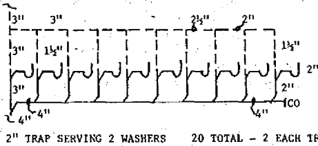
2" TRAP SERVING 2 WASHERS 20 TOTAL - 2 EACH TRAP
