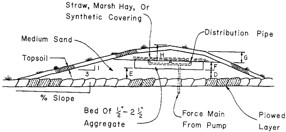
Cross Section Of A Mound System Using A Bed For The Absorption Area
