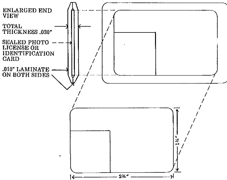
FIGURE 3 Laminate Specifications
