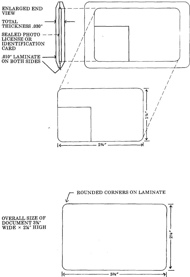
FIGURE 3 Laminate Specifications
