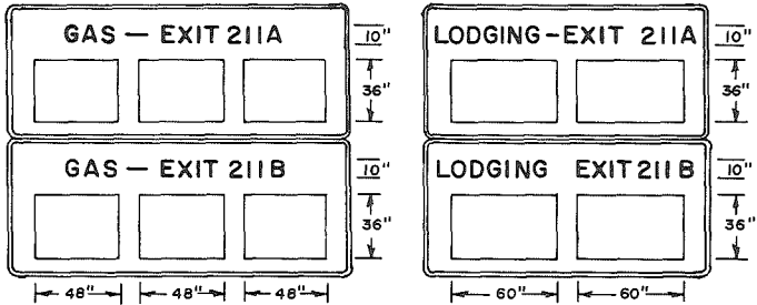
DOUBLE EXIT INTERCHANGE
