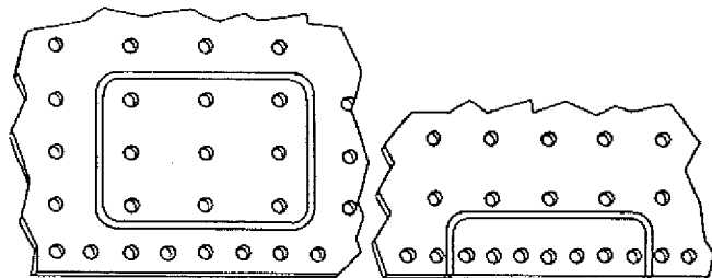
FLUSH PATCHES IN STAYED AREAS
