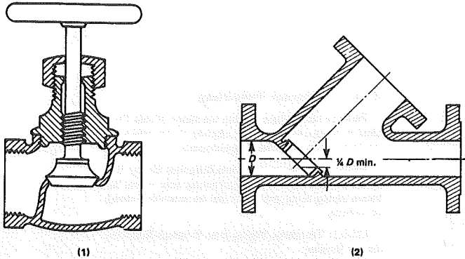
FIG. 122.1.7(C) TYPICAL GLOBE VALVES
