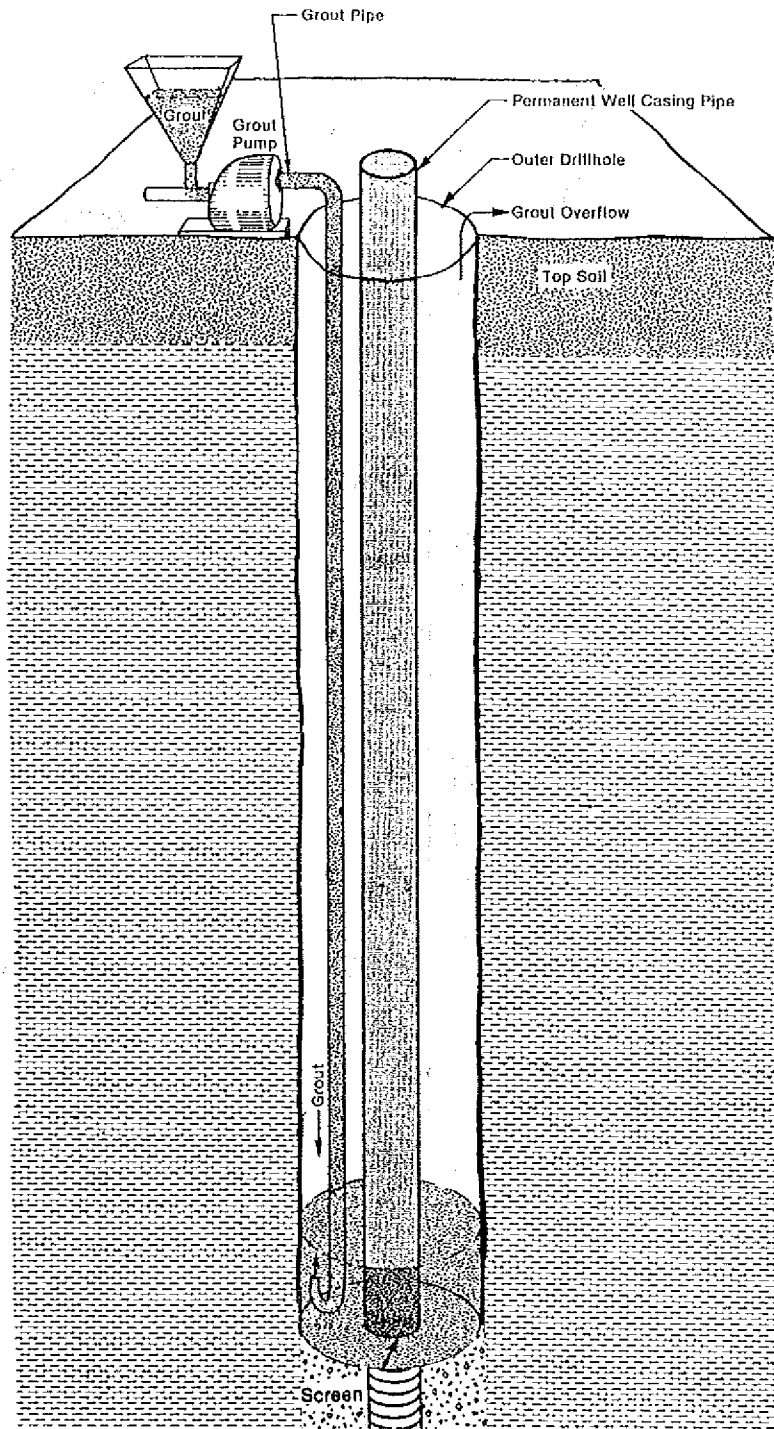
Figure 3. Conductor (tremie) pipe — pumped method
