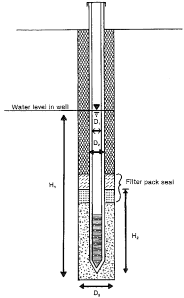
IN PIEZOMETER
