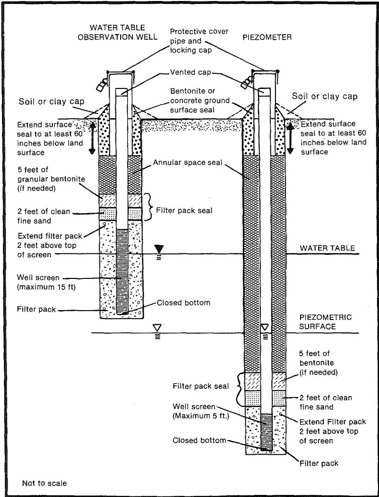
Typical water table observation well and piezometer construction details.
