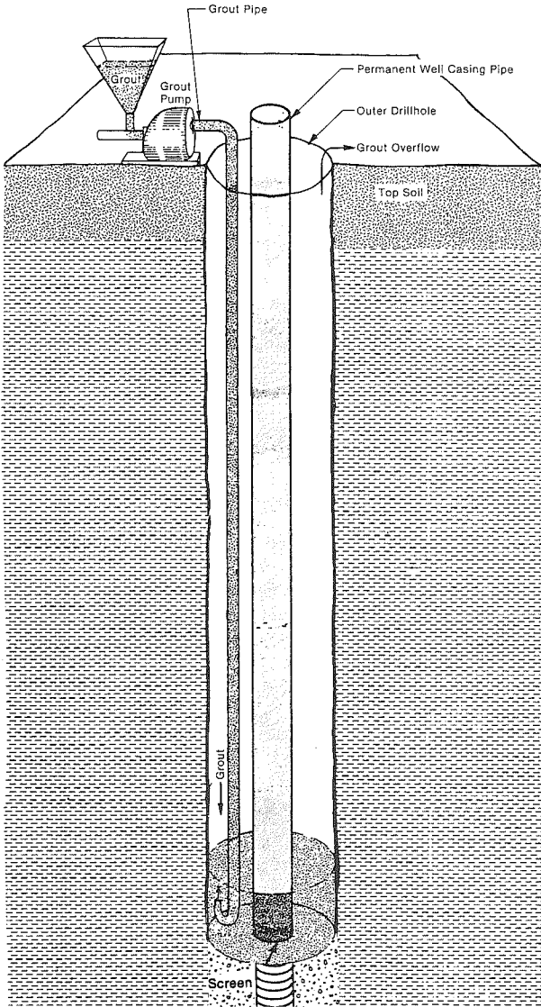
Figure 3. Conductor (tremie) pipe — pumped method
