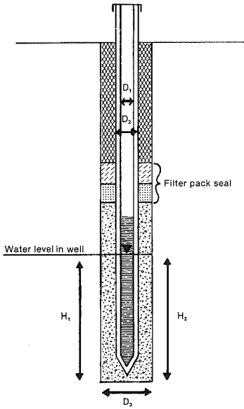
IN WATER TABLE OBSERVATION WELL
