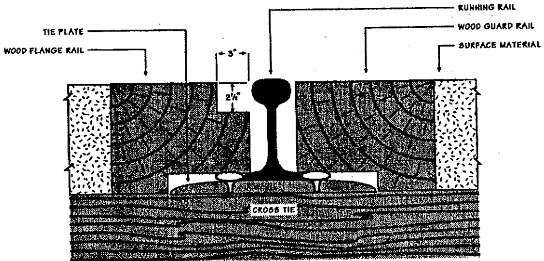
CROSS SECTION
