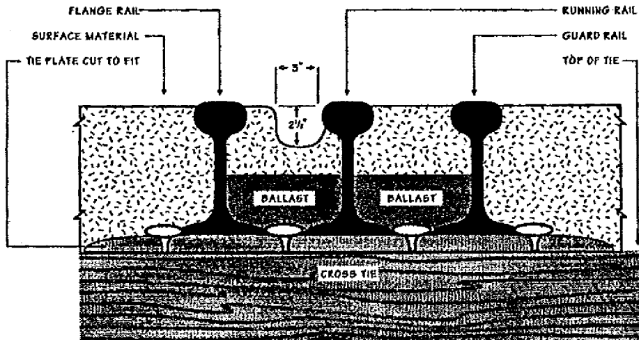
3 RAIL — STEEL CROSS SECTION
