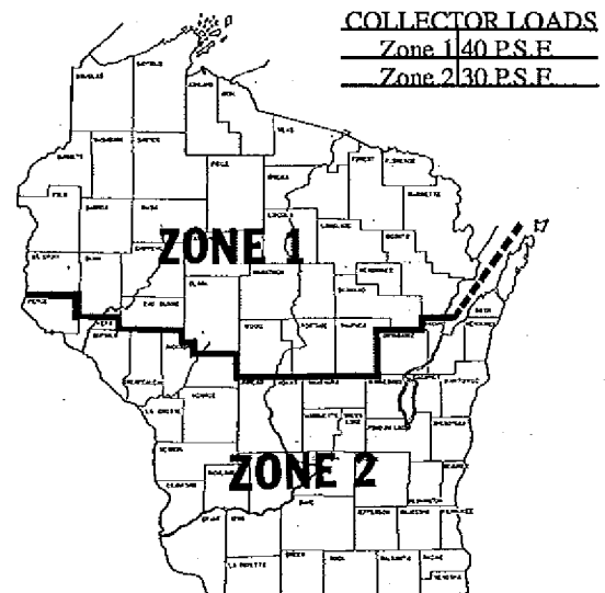
Zone Map for Collector Loads
