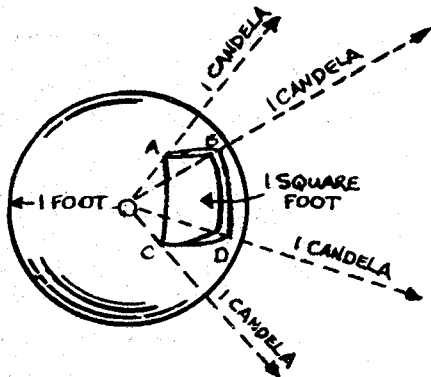
Figure D-1. Relationship between candelas, lumens and footcandles. A uniform point source (luminous intensity or candlepower = 1 candela) is shown at the center of a sphere of 1-foot radius. It is assumed that the sphere is perfectly transparent (i.e., has 0 reflectance). The illumination at any point on the sphere is 1 footcandle (1 lumen per square foot). The solid angle subtended by the area, A, B, C, D is 1 steradian. The flux density is, therefore, 1 lumen per steradian, which corresponds to a luminous intensity of 1 candela, as originally assumed. The sphere has a total area of 12.57 (4) square feet, and there is a luminous flux of 1 lumen falling on each square foot. Thus the source provides a total of 12.57 lumens.
