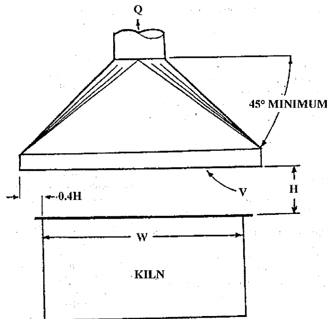
FIGURE 32.24 CANOPY HOOD
