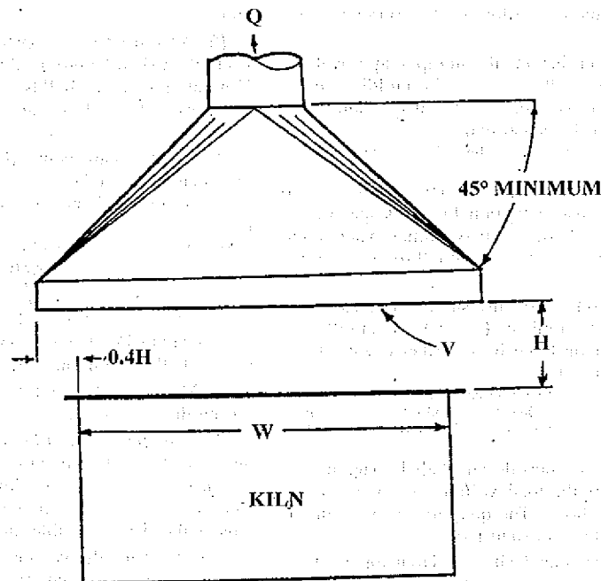
FIGURE 32.24 CANOPY HOOD
