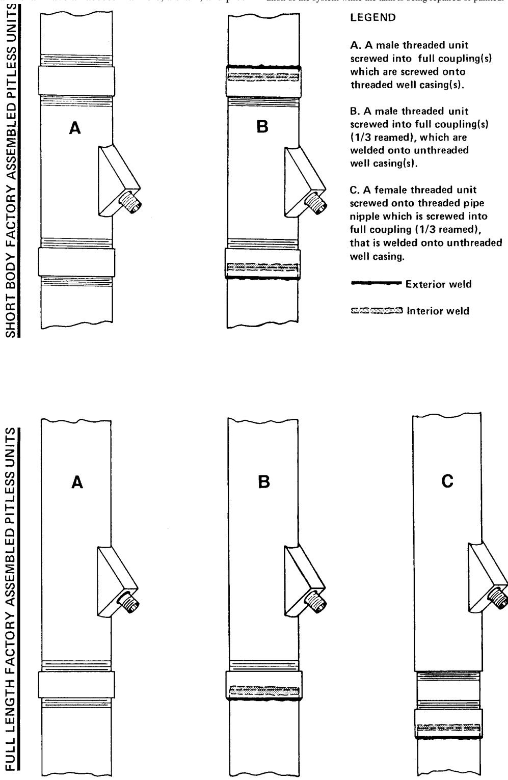
Figure 30. Pitless unit connections for wells with steel well casing pipe. NOTE: A well casing pipe nipple, 1/2 threaded–1/2 beveled may be used in lieu of a full pipe coupling.
