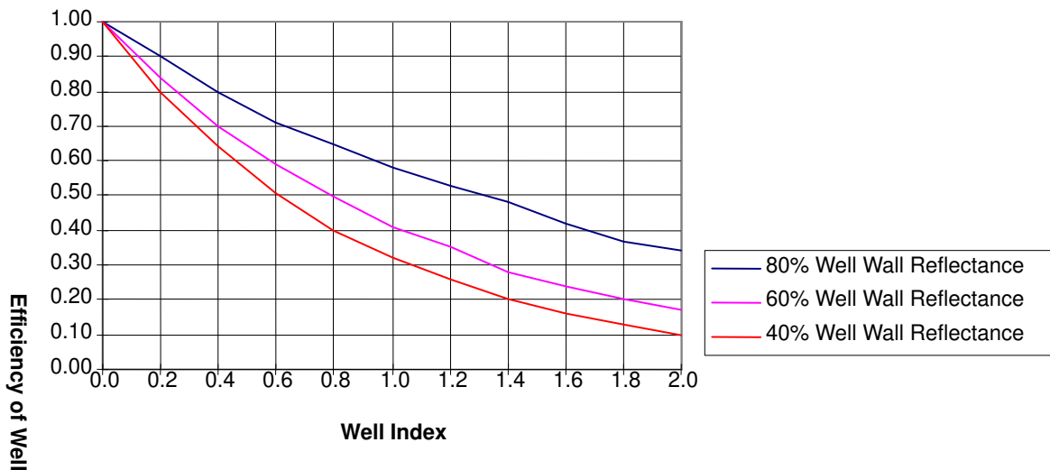
Figure 63.1005 Well Efficiency
