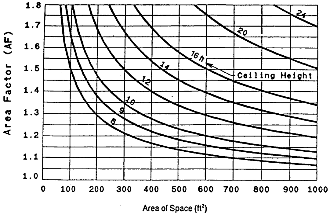
Figure 63.1049 Area Factor
