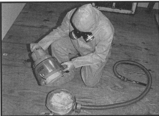
Figure 11.16a Remove the HEPA Vacuum Filters and Disassemble the Vacuum With a Plastic Sheet Underneath.
