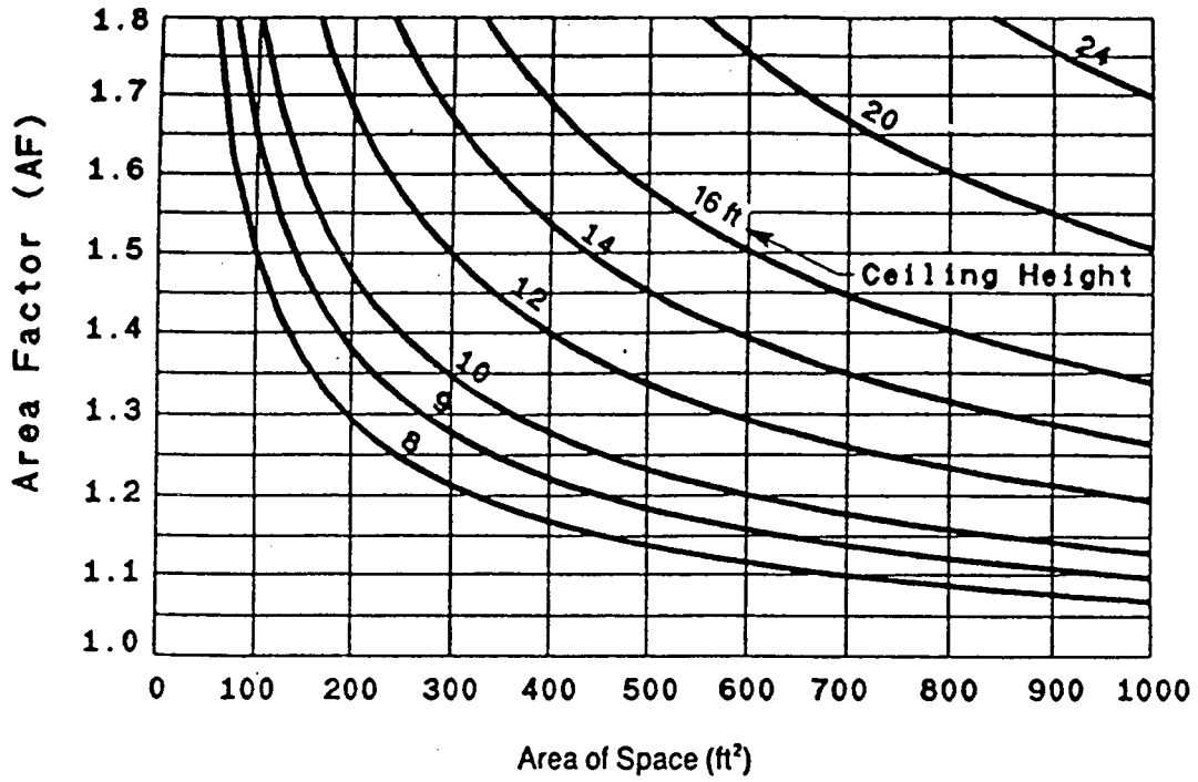
Figure 63.1049 Area Factor
