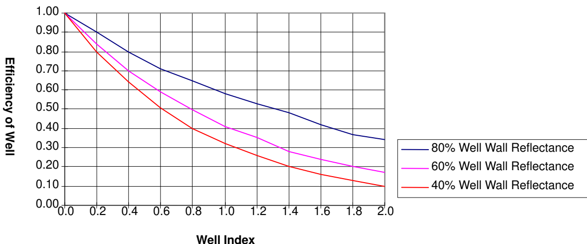
Figure 63.1005 Well Efficiency
