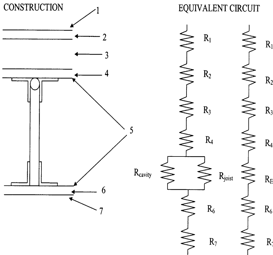
Calculation Procedure for Thermal Resistance of a Typical Roof Assembly
