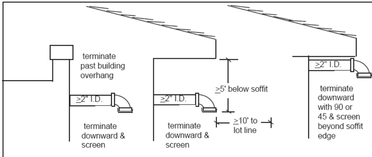
VENTS TERMINATING THROUGH WALLS
