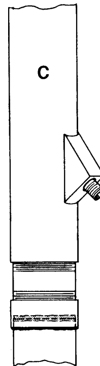
Figure 30. Pitless unit connections for wells with steel well casing pipe. NOTE: A well casing pipe nipple, 1/2 threaded–1/2 beveled may be used in lieu of a full pipe coupling.
